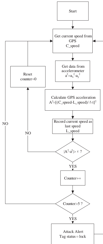
Figure 3: Flow chart for detecting GPS spoofing attack
